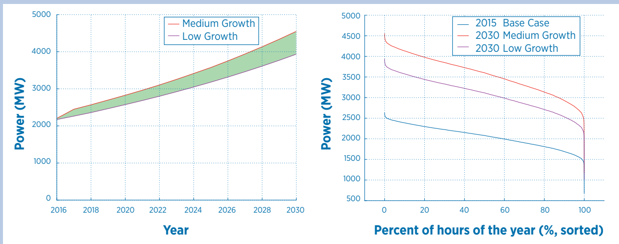
Figure 29: Power demand projections to 2030 (left) and load duration curves (right)
