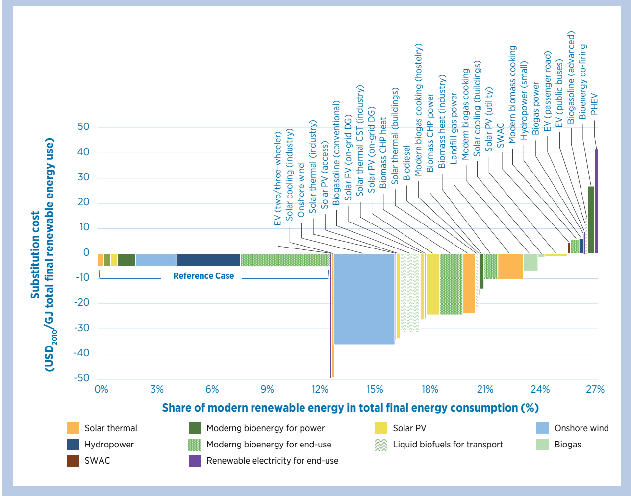
Figure 41: Renewable energy cost-supply curve by renewable energy resource, business perspective, 2030
