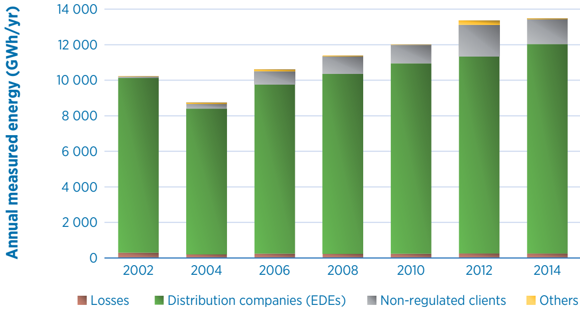
Figure 16: Annual energy measured by SENI for selected years (2002-2014)
