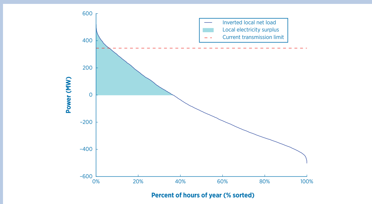
Figure 36: Local net load for South region
